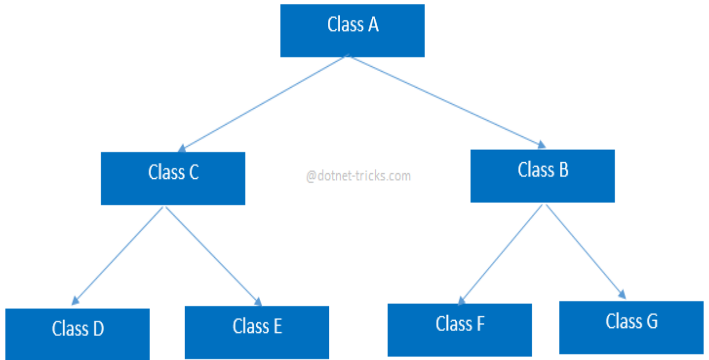
Hierarchical Inheritance
